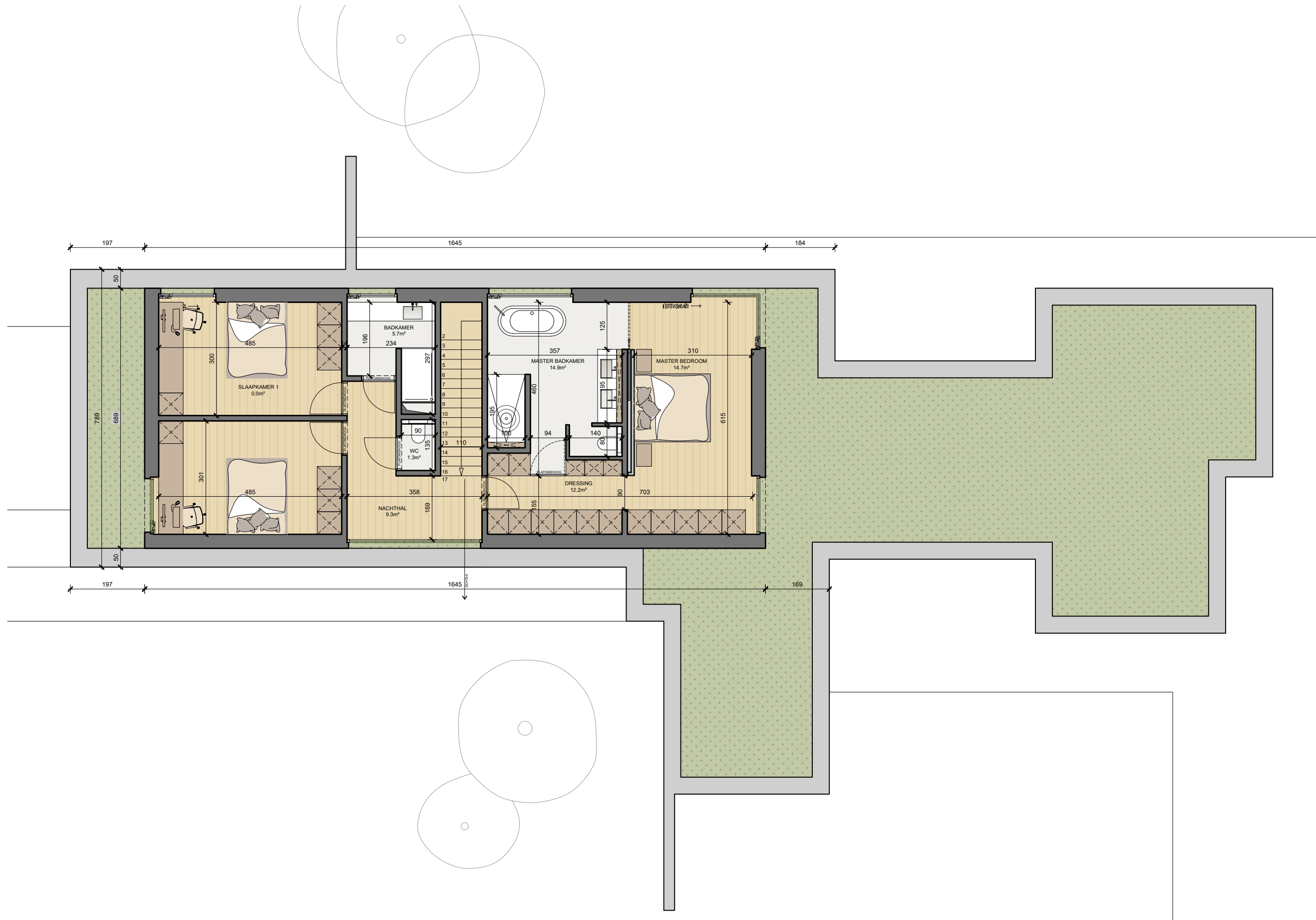
PLAN NIVEAU +1 WONING - BRUTO OPP. : 113.3m 2
